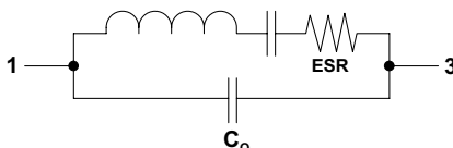
Crystal Equivalent Circuit
