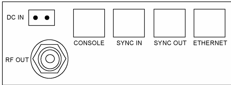
Figure 2. SEM910 Back Panel Diagram
