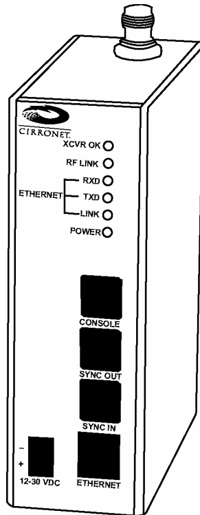
Figure 3. SEM910D Front Panel Diagram
