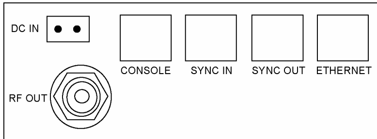
Figure 5. SEM910X Back Panel Diagram
