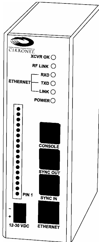
Figure 6. SEM910DX Front Panel Diagram
